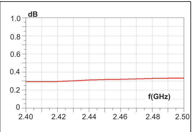
Figure 10. Amplitude imbalance
