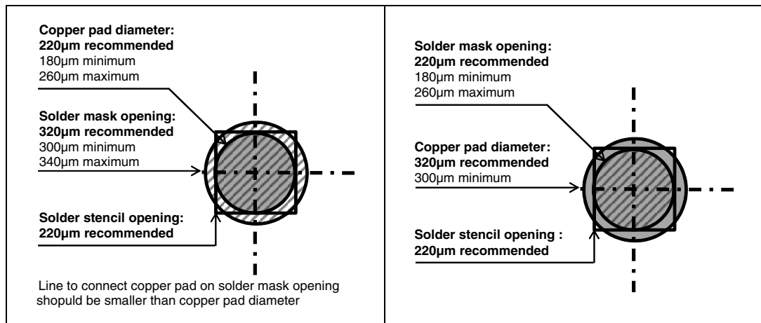
Figure 23. Footprint - non solder mask defined Figure 24. Footprint - solder mask defined
