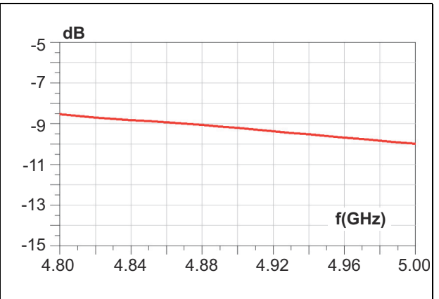
Figure 6. H2 filtering
