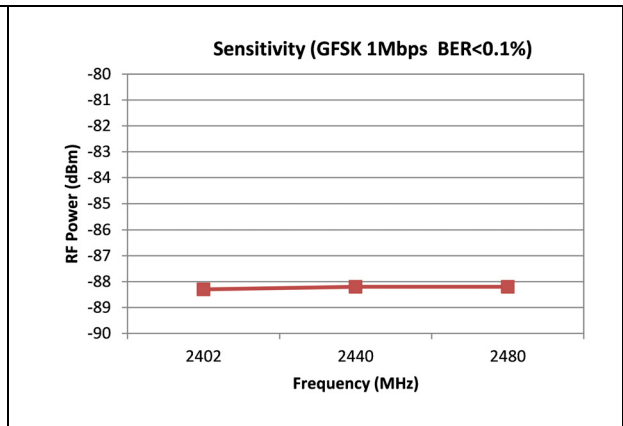
Figure 15. Sensitivity
