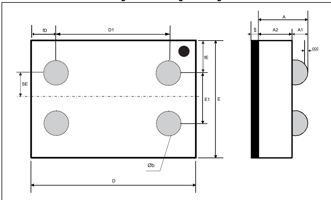
Figure 22. Package drawing
