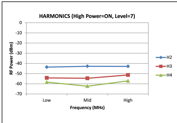
Figure 14. Harmonics
