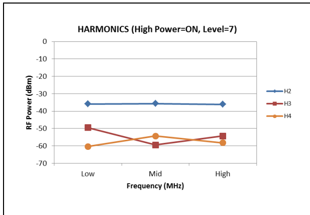
Figure 19. Harmonics
