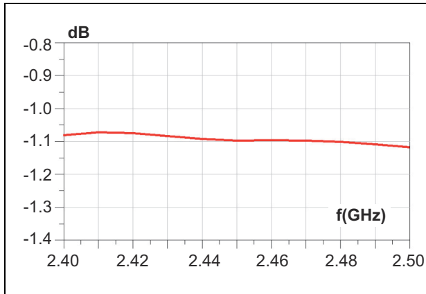
Figure 5. Insertion loss
