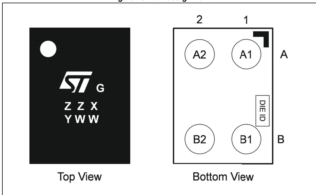
Figure 25. Ball assignment
