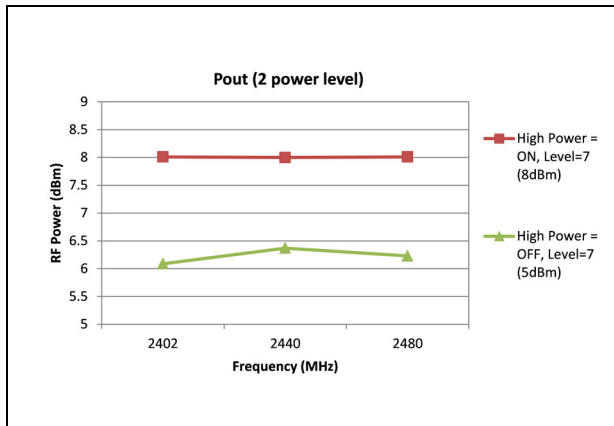
Figure 16. Pout
