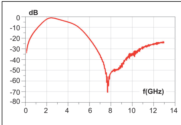
Figure 3. Differential transmission
