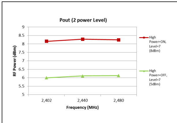
Figure 21. Pout
