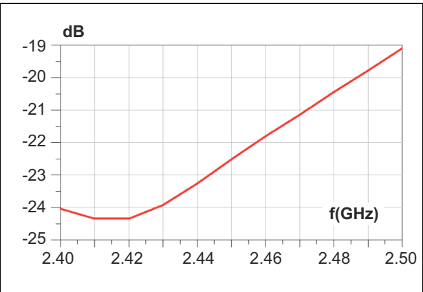
Figure 4. Return loss
