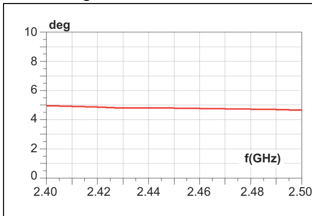
Figure 11. Phase imbalance
